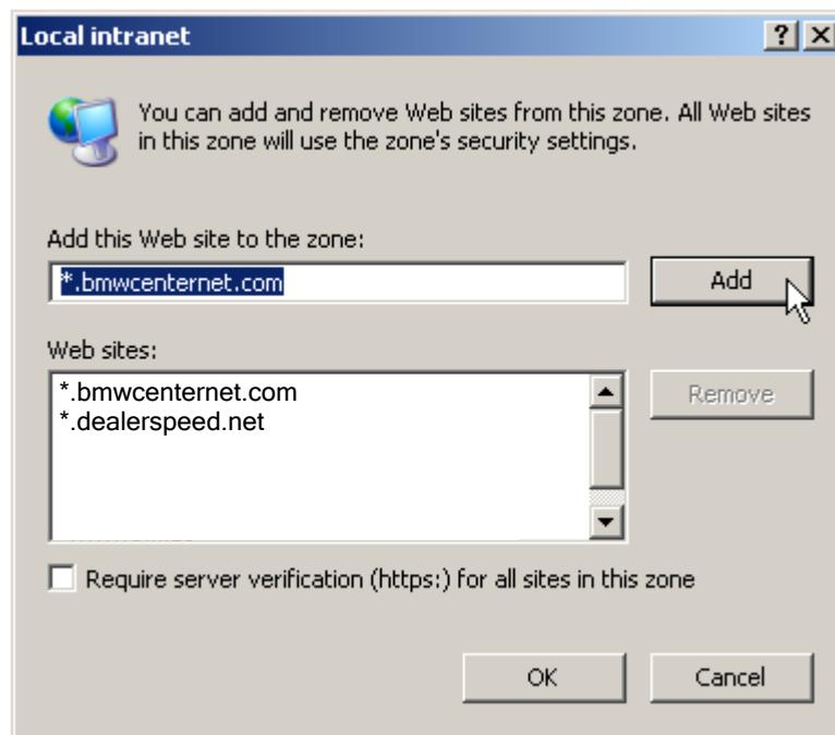
Fig. 3: Internet Explorer - Local Intranet Zone Settings
